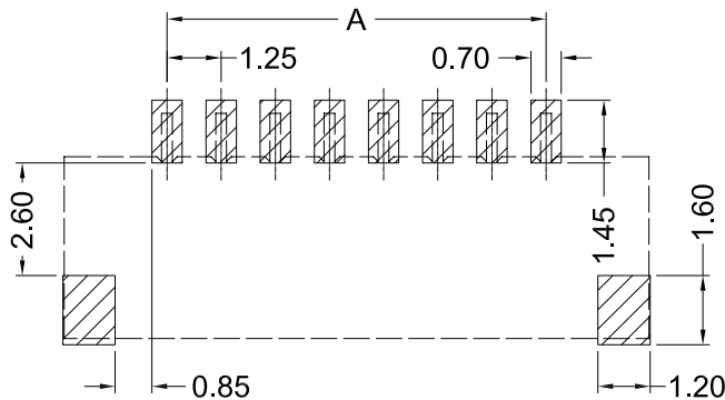
Recommended P.C.B Layout General Tolerance \pm 0.05
