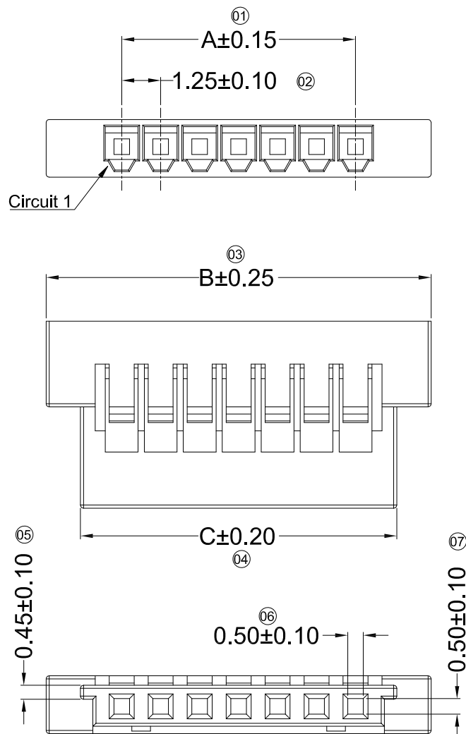
4P~30P Double Salient Scale 1:5
