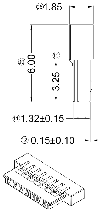
4P~30P Double Salient Scale 1:5
