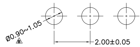
RECOMMENDED P.C.B LAYOUT (Thickness=1.60mm)
