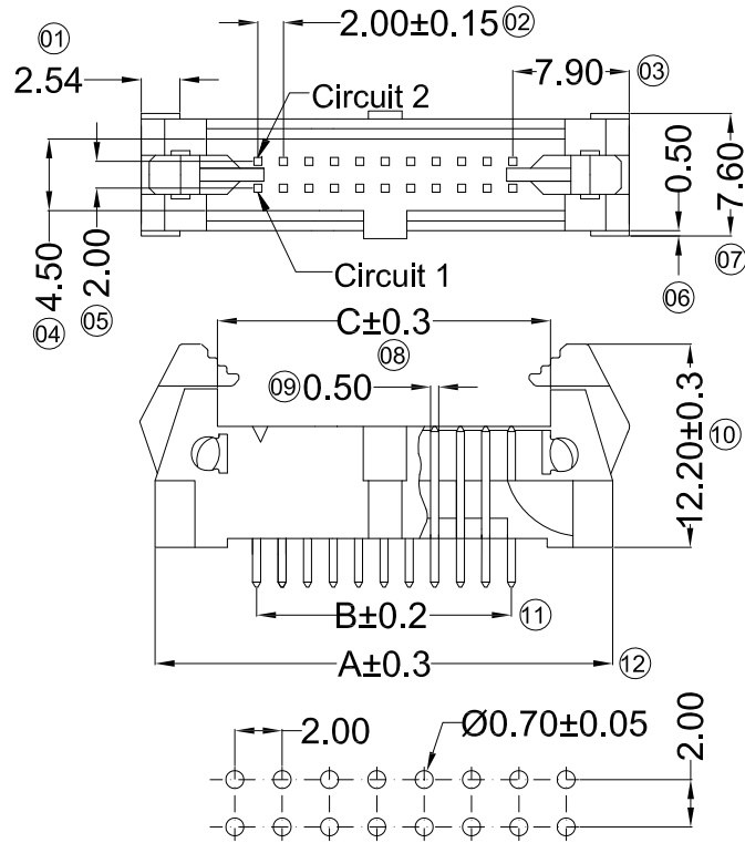
Recommand PCB Layout
